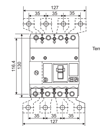
4-Pole with spreaders
