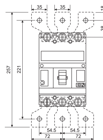
3-Pole with spreaders
