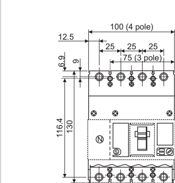
3-Pole, 4-Pole
