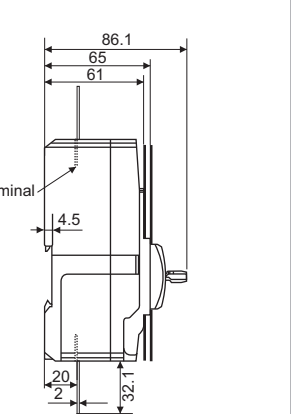
3-Pole, 4-Pole
