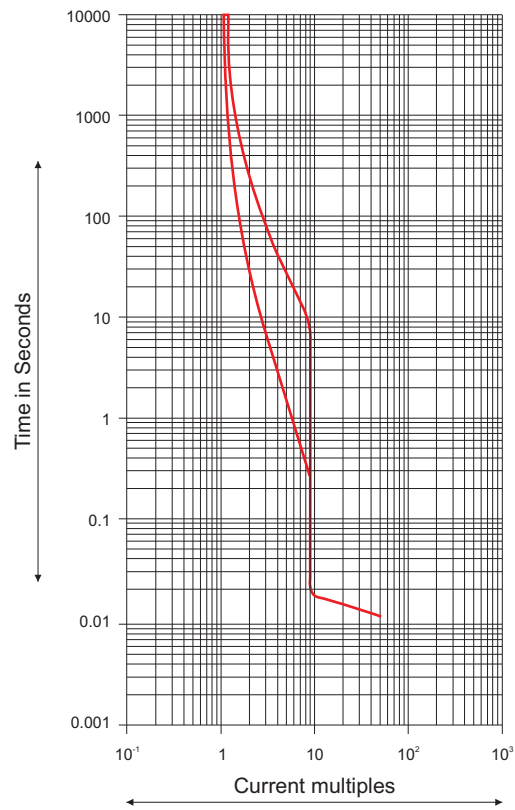
DU100/DU100H
