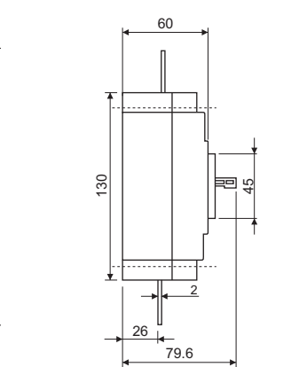
3-Pole
