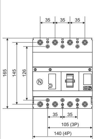
3-Pole, 4-Pole
