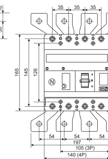
4-Pole with spreaders
