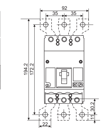
3-Pole with spreaders
