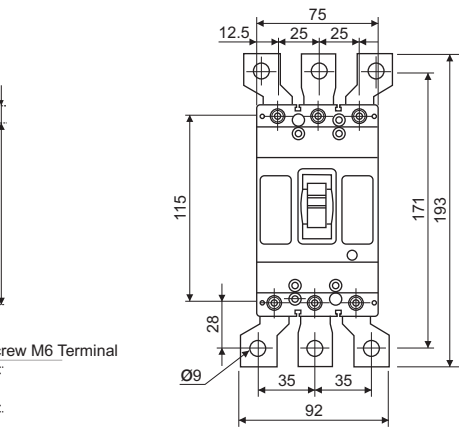
3-Pole with spreaders
