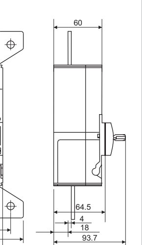
3-Pole, 4-Pole
