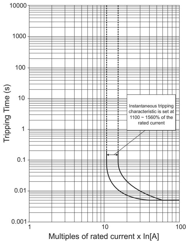
Type MOG - H1M (0.16A - 32A)
